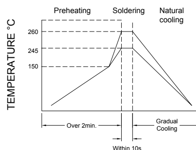
Figure 2. Wave Soldering
